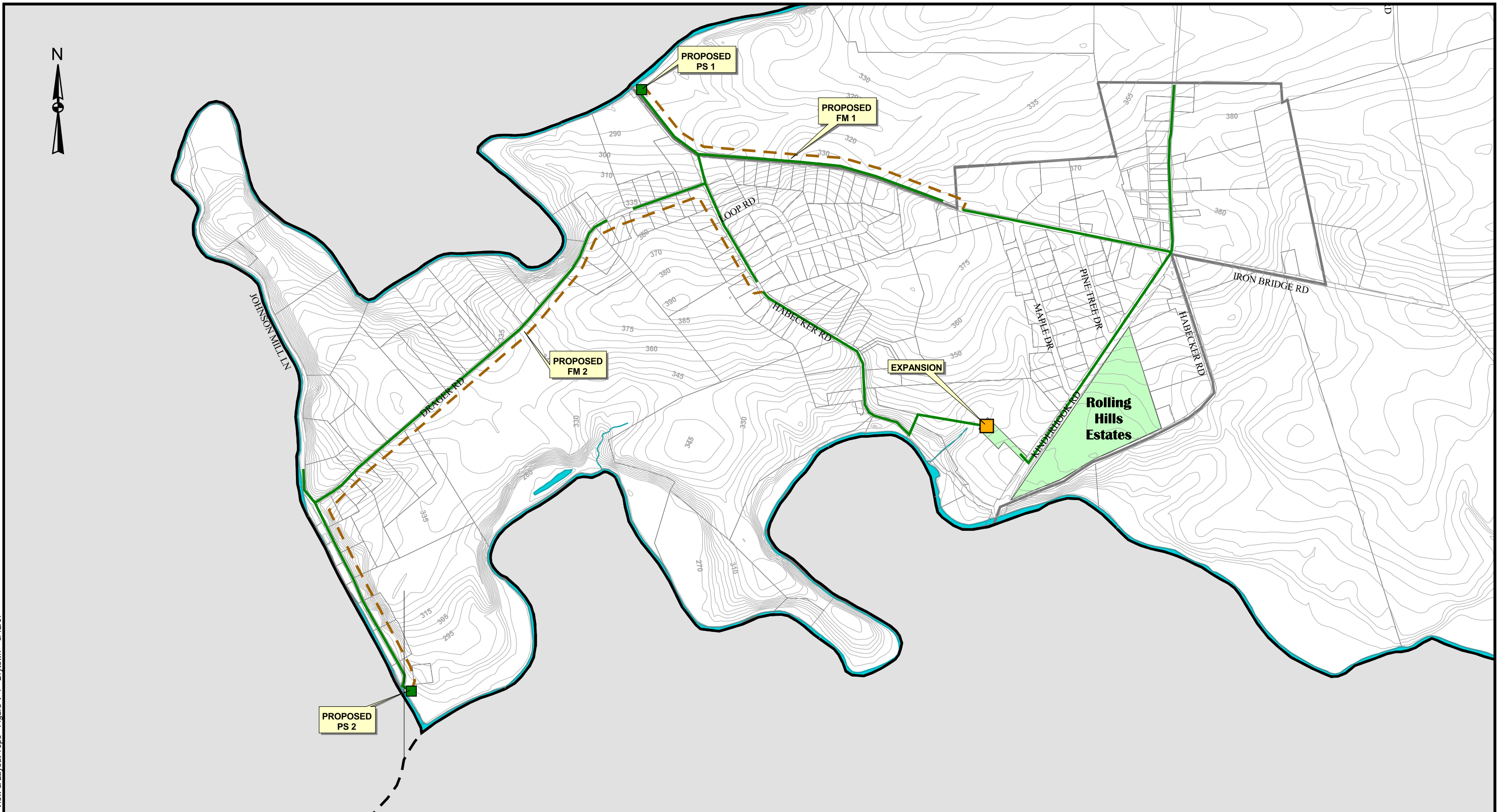
FIGURE V-1 Newtown Area Sewer Extension to Rolling Hills Mobile Home Park WWTP
